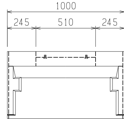
L = 1000
