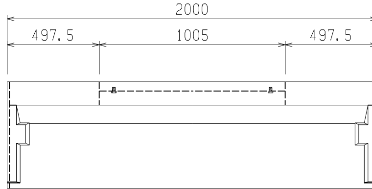
L = 2000
