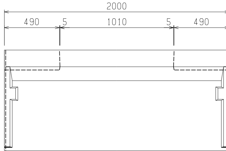
L = 2000
